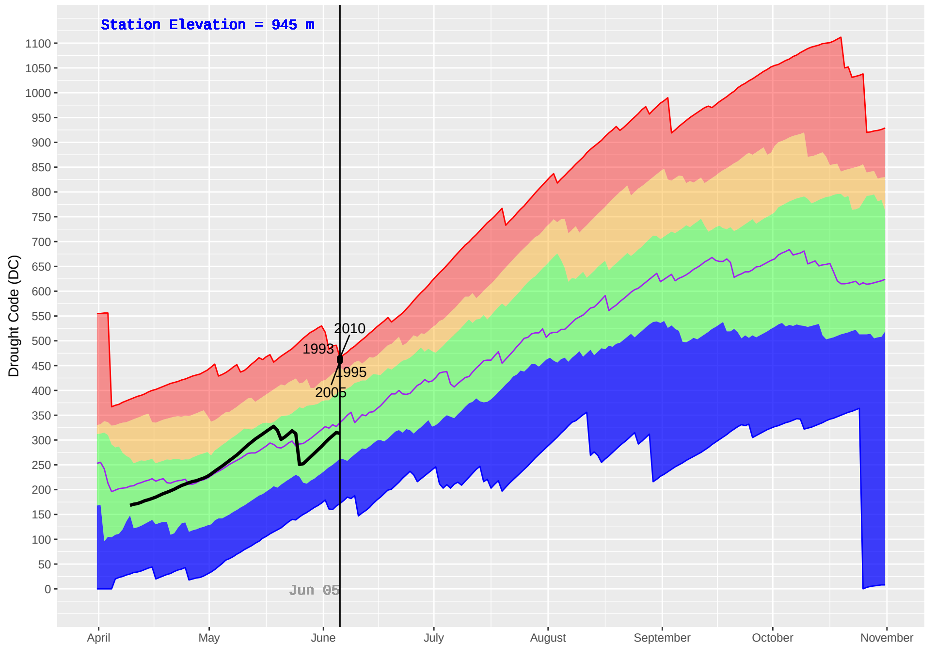
TATLA LAKE HUB (208) : Historical (1980–2018) and Current (2019) Daily Drought Code (DC)
