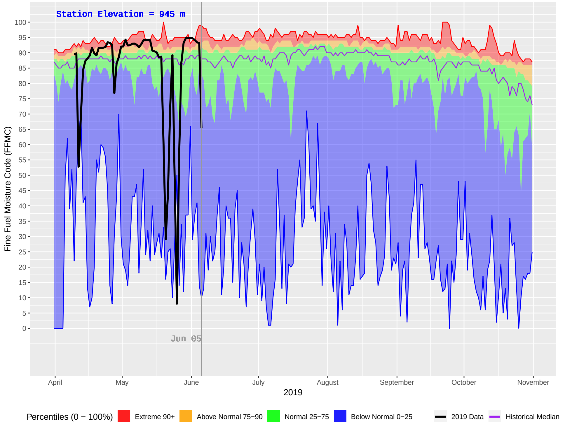
TATLA LAKE HUB (208) : Historical (1980–2018) and Current (2019) Daily Fine Fuel Moisture Code (FFMC)
