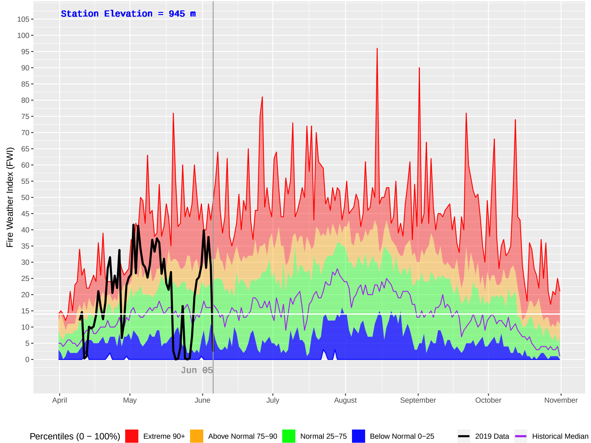
TATLA LAKE HUB (208) : Historical (1980–2018) and Current (2019) Daily Fire Weather Index (FWI)
