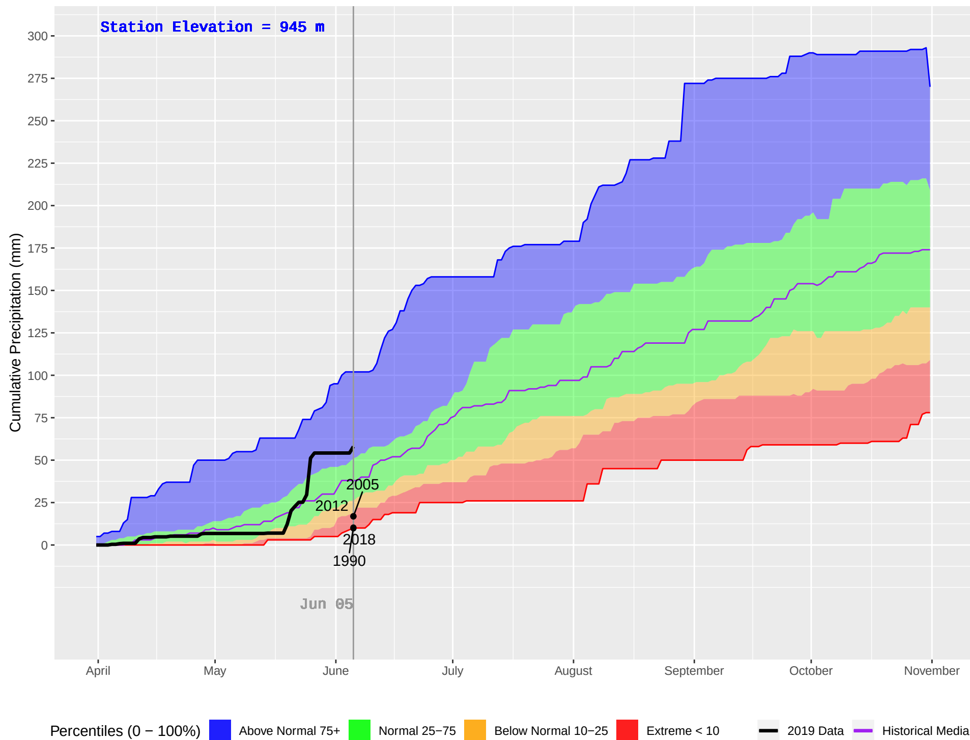
TATLA LAKE HUB (208) : Historical (1980–2018), Current (2019) Daily Cumulative Precipitation
