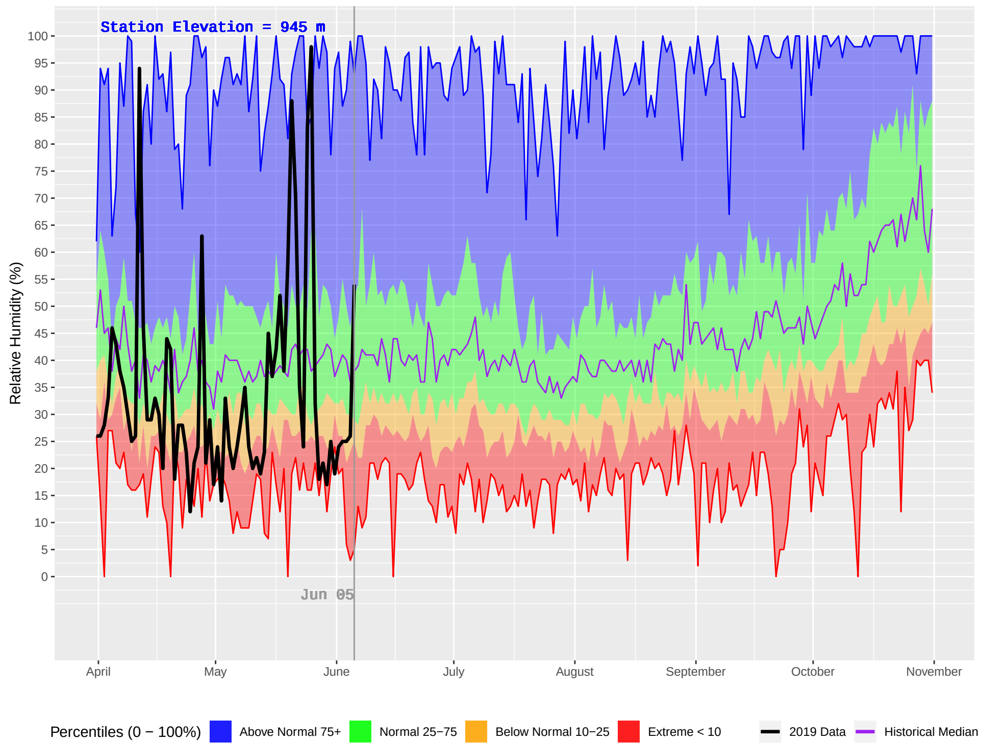
TATLA LAKE HUB (208) : Historical (1980–2018) and Current (2019) Daily Relative Humidity
