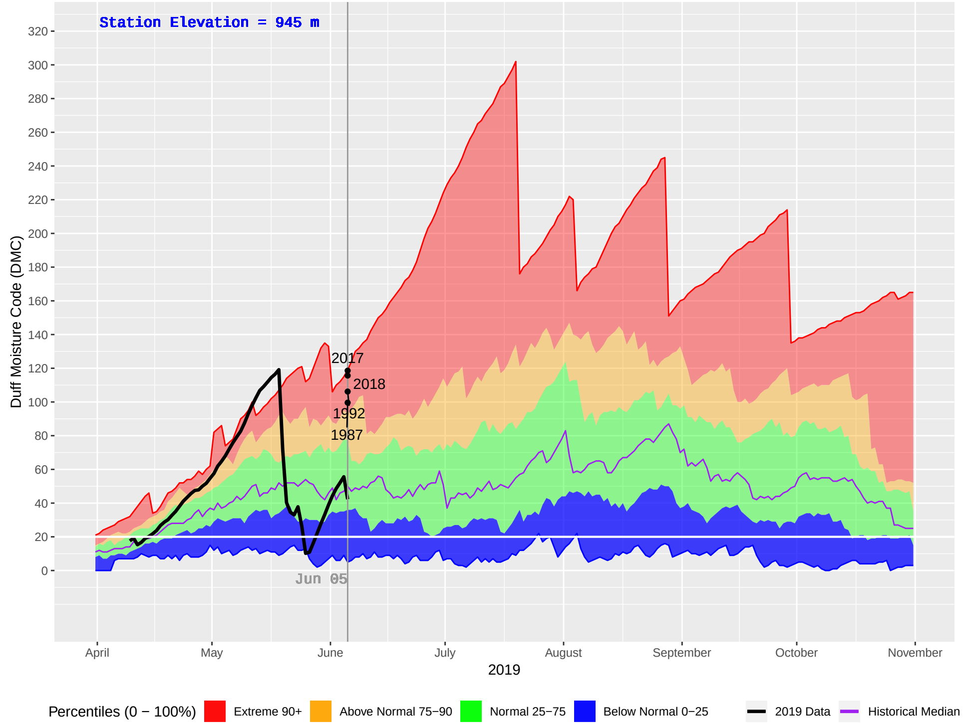
TATLA LAKE HUB (208) : Historical (1980–2018), Current (2019) Daily Duff Moisture Code (DMC)
