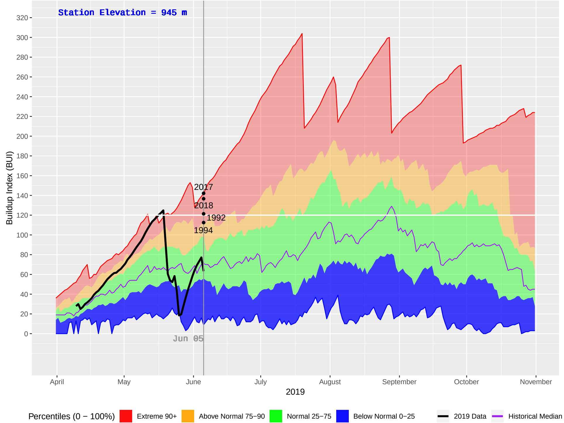
TATLA LAKE HUB (208) : Historical (1980–2018), Current (2019) Daily Buildup Index (BUI)
