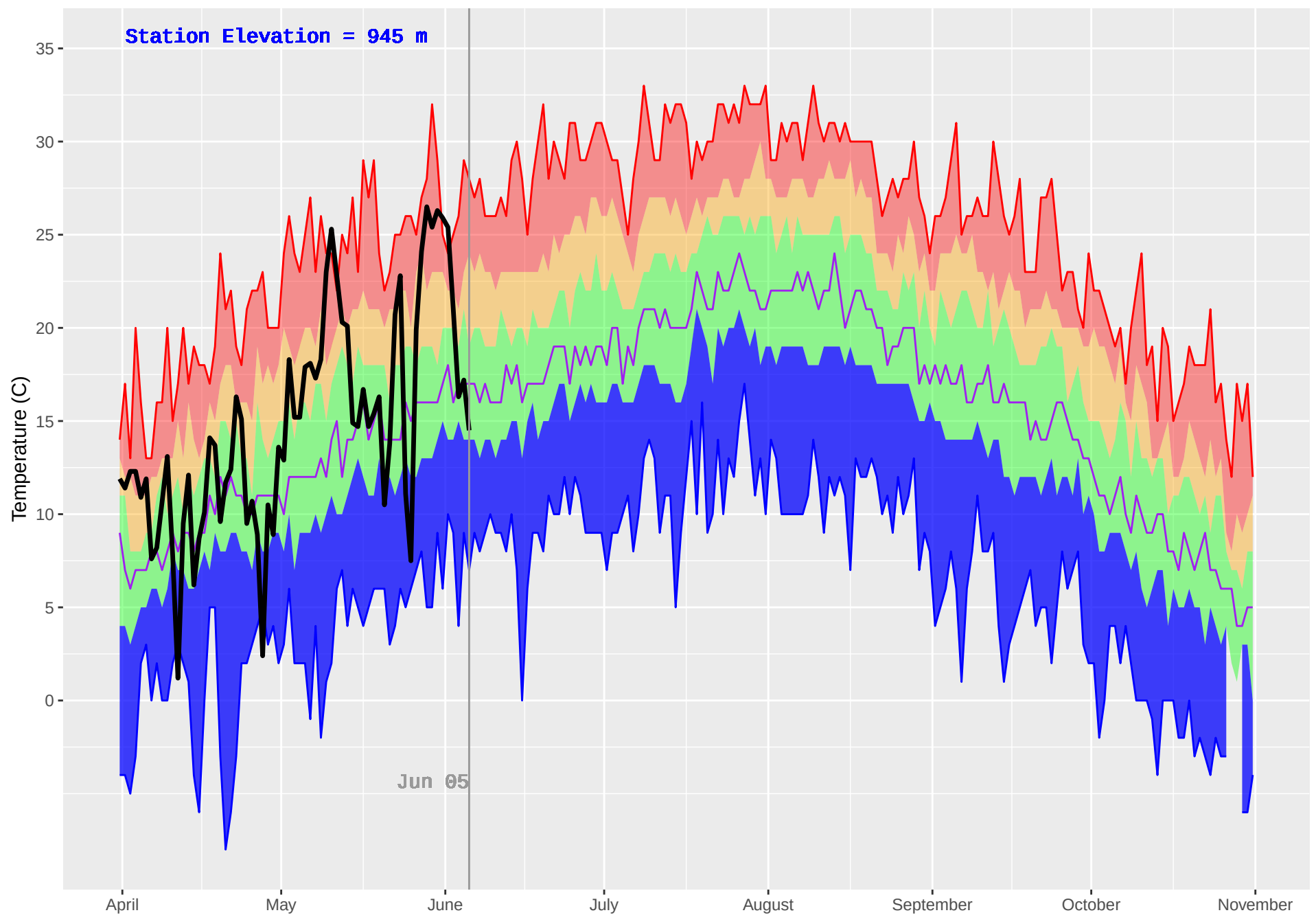
TATLA LAKE HUB (208) : Historical (1980–2018) and Current (2019) Daily Temperature
